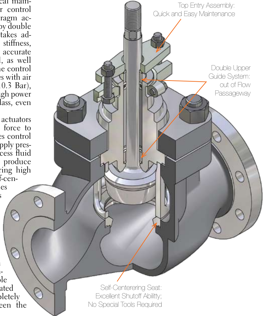
GL \bar{5} SERIES – BODY SUB-ASSEMBLY (FIGURE 1)
