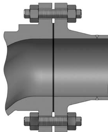
SEPARABLE END AND BONNET FLANGES (FIGURE 8)
